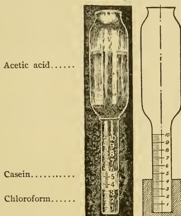
Tubes for Hart's Casein Test.
